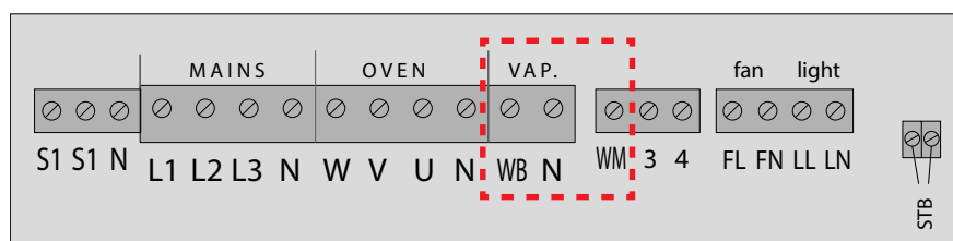
Vaporiser connection
