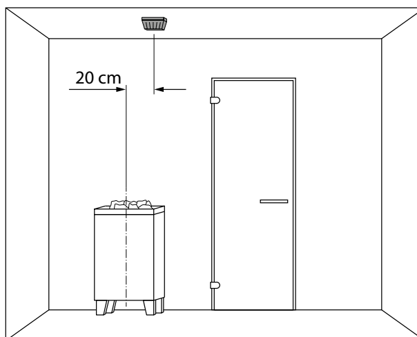
📐 Installation configuration above the heater
